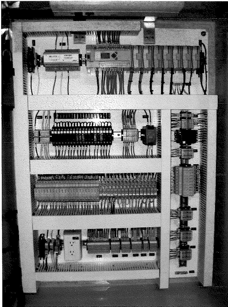
NRO Plant Chemical Pump Control Panel Back Panel
