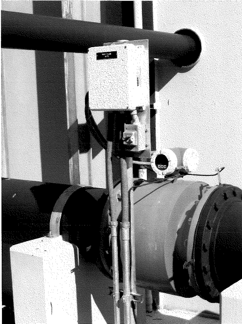
Gateway WWTP – Flowmeter Installation
