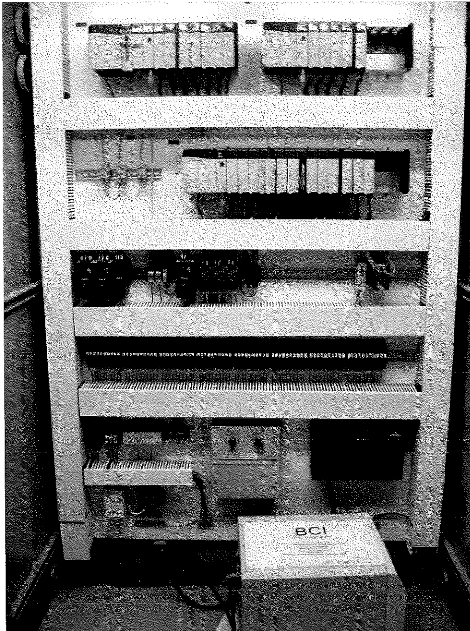
Gateway WWTP - PLC Control Panel 1
