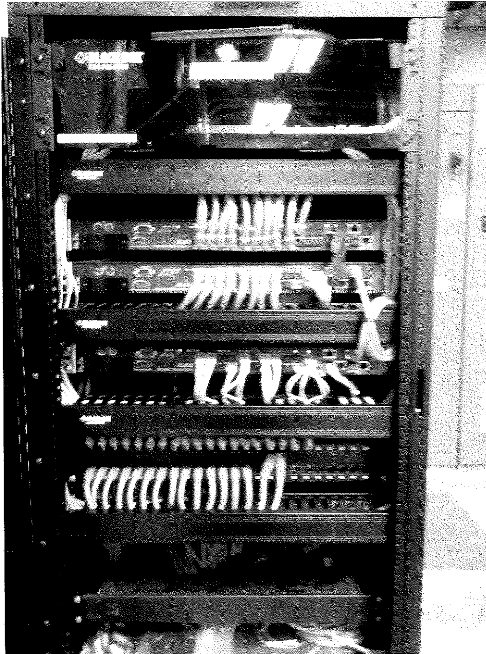
NRO Plant – New MCC Room Fiber Optic Network Panel
