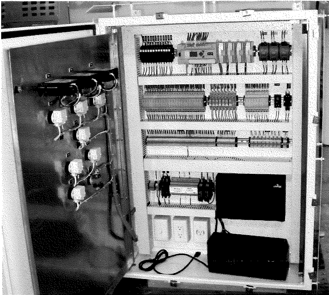
NRO Well Field – Pump Control Panel Back Panel
