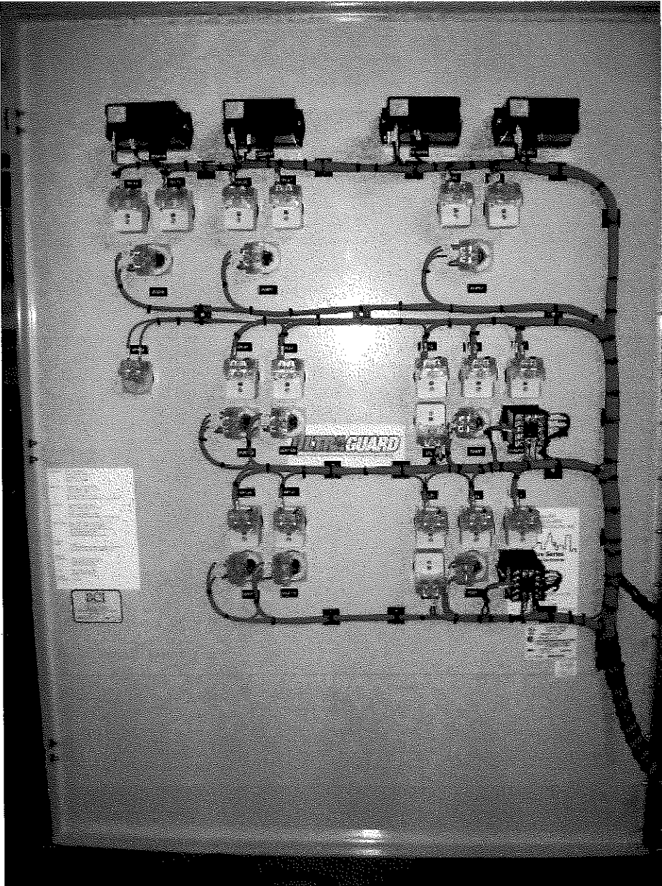
NRO Plant Chemical Pump Panel Door (Back)
