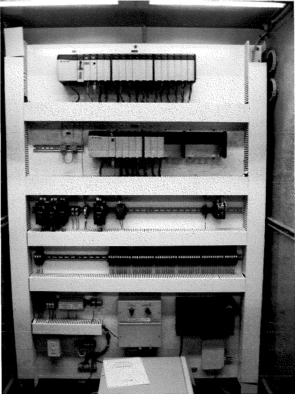
Gateway WWTP - PLC Control Panel 2
