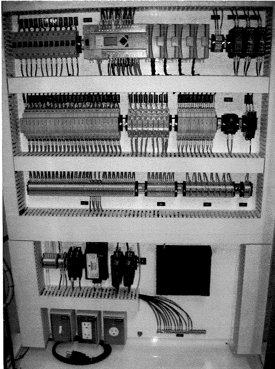
NRO Well Field – Pump Control Panel (Back Panel)
