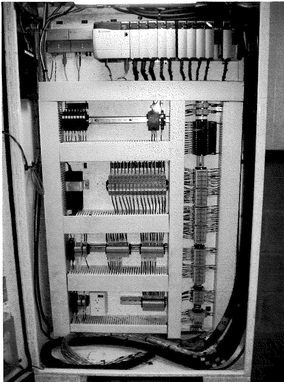
NRO Plant Train 3&4 Control Panel
