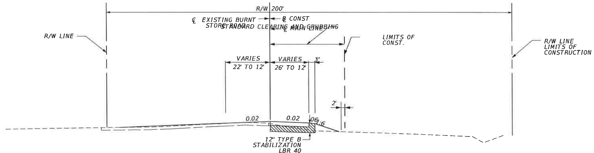
TYPICAL SECTION BURNT STORE ROAD STA. 1315+40.00 TO 1321+00.00 NB & SB WIDENING SEE TYPICAL SECTION DETAILS NORTH BOUND LANES
