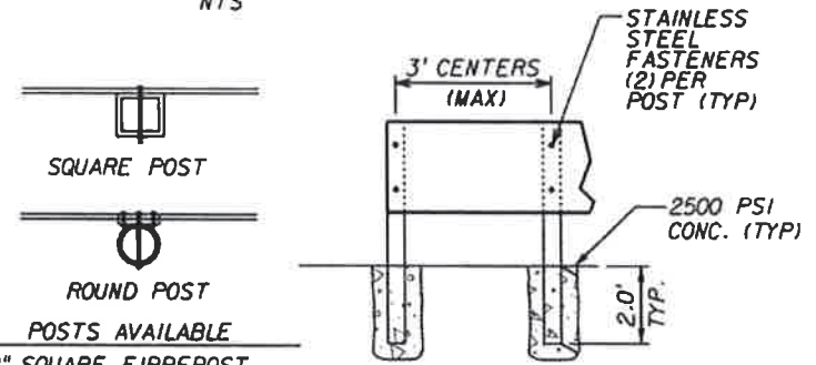
POST MOUNTED DETAIL FOR FIBERGLASS SKIMMER NTS
