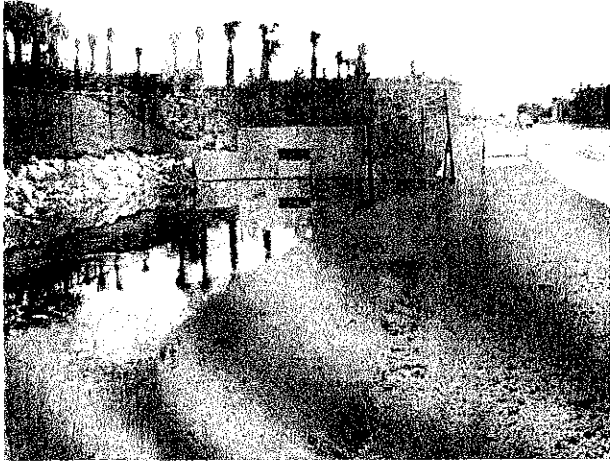
Storm water management control structure along the newly completed Three Oaks Parkway Extension south of Corkscrew Road.
