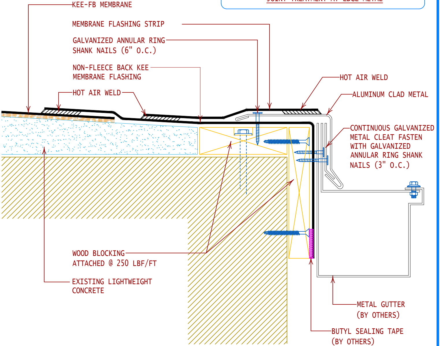
GUTTER EDGE FLASHING LIGHTWEIGHT CONCRETE
