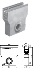
FILCOTEN Tec Sump Unit 100
