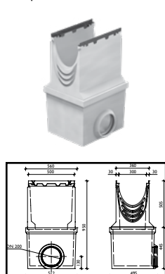
FILCOTEN Pro 300 Sump Kit with Silt Bucket
