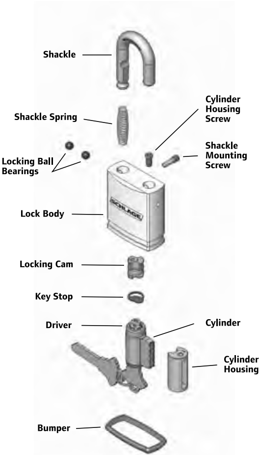
Conventional Key-in-Lever
