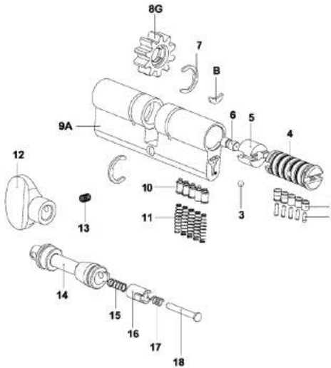
Euro Single w/Thumb Turn
