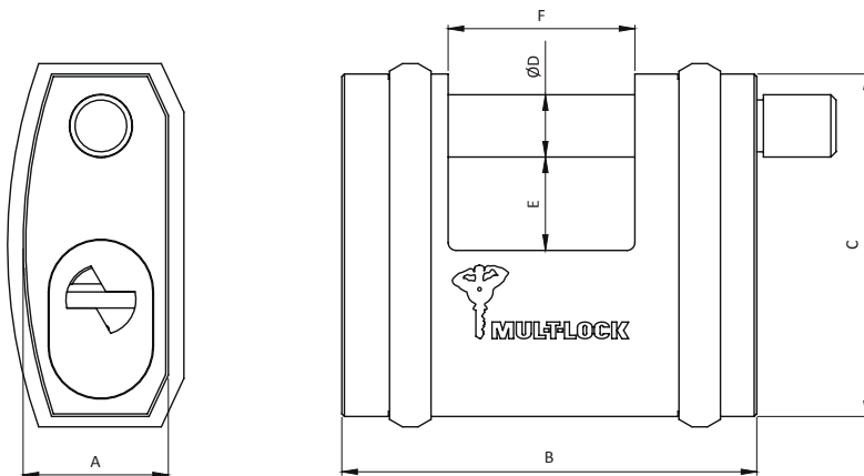
* NE12SB Measurements - New Size
