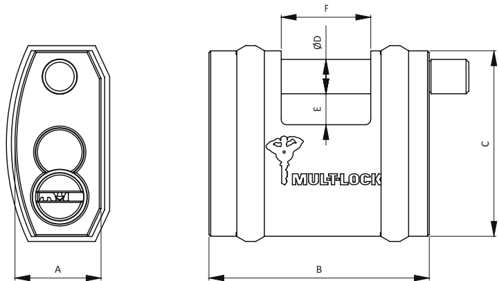
NG10SB Measurements
