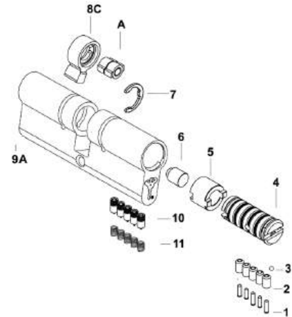
Euro Double (Key on both sides)
