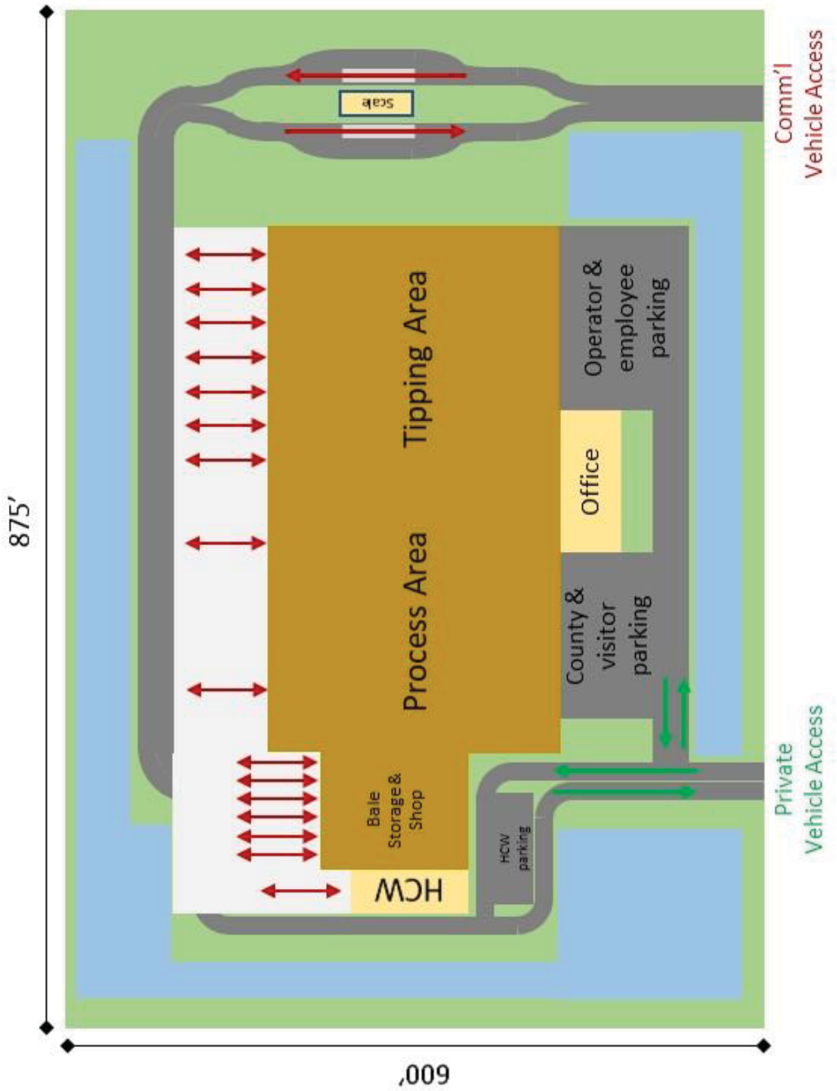
Figure 1: Generic Conceptual Layout – County-wide SSR MRF
