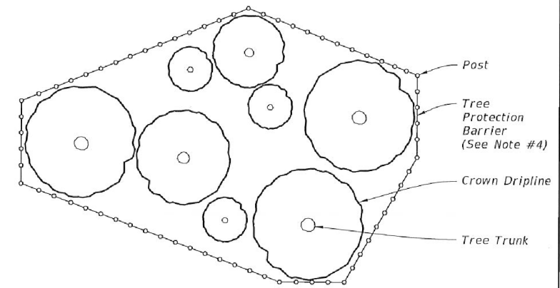
PLAN PROTECTION BARRIER FOR TREE GROUPINGS
