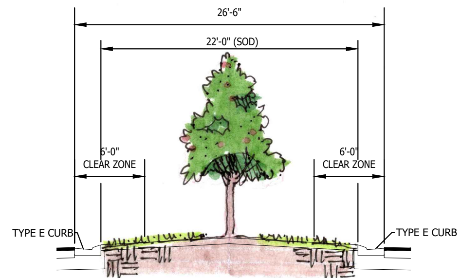
TYPICAL MEDIAN SECTION 2 SCALE: 1/8" = 1'-0"
