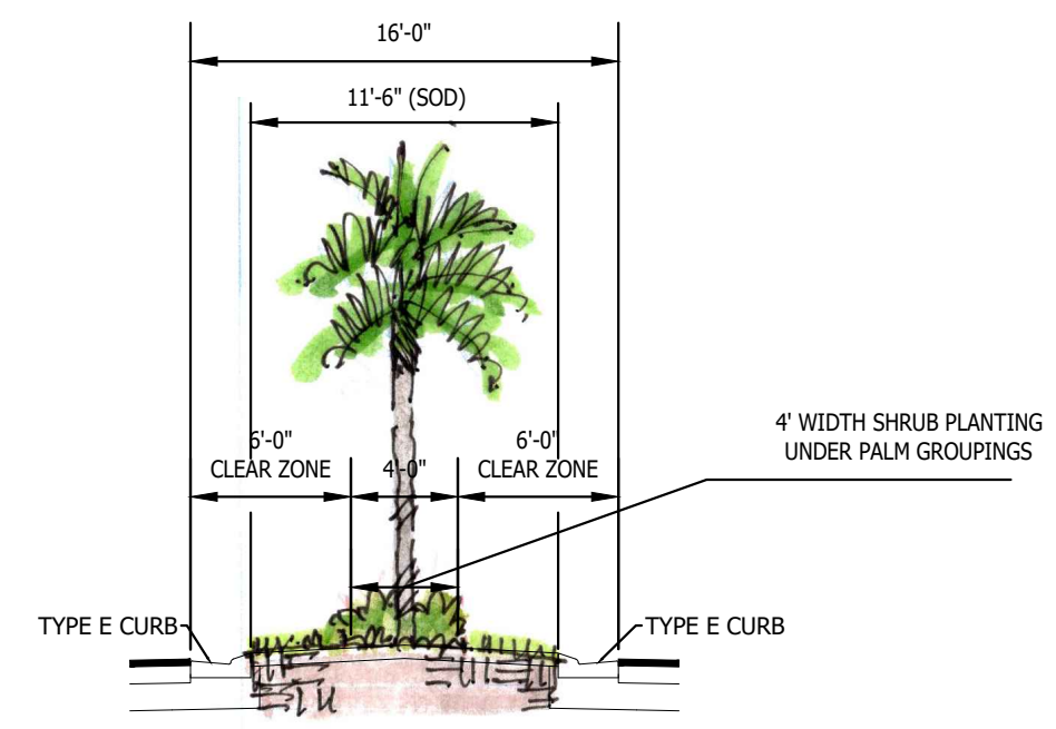
TYPICAL MEDIAN SECTION 3 SCALE: 1/8" = 1'-0"
