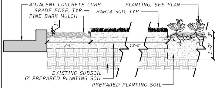
A ROAD ISLAND EDGE CONDITIONS NTS P-BU-03
