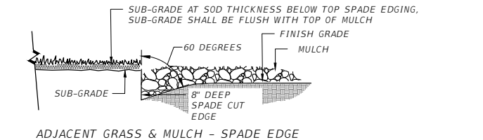
D SPADE EDGE CONDITION NTS P-BU-07
