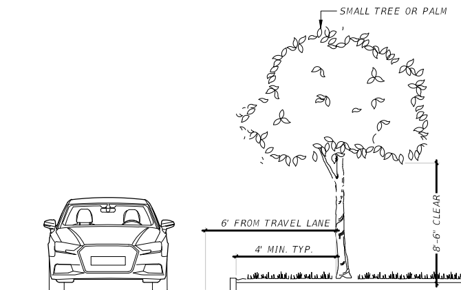
C LATERAL OFFSET TO TREES IN MEDIAN NTS P-BU-08
