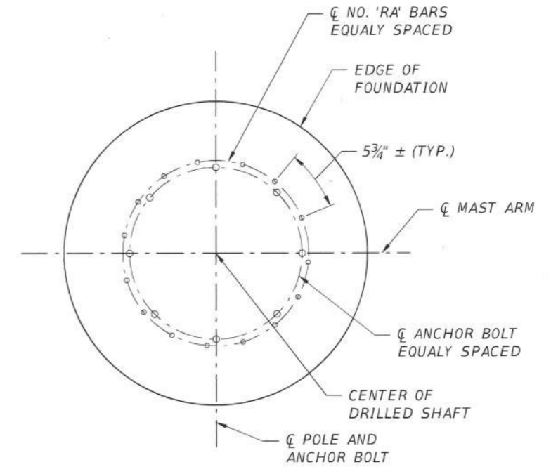
DRILLED SHAFT PLAN SHOWING ANCHOR BOLT & REINFORCING DETAILS
