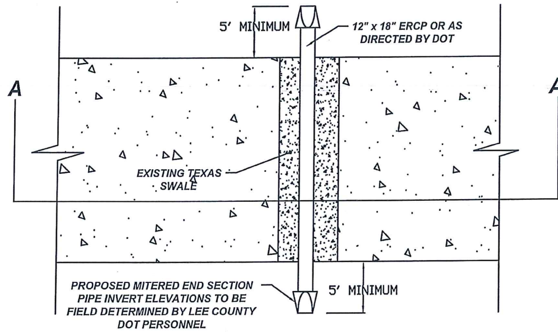
PLAN VIEW
