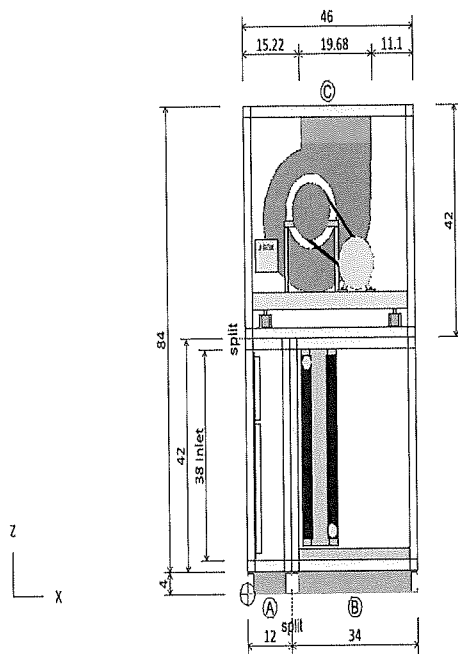
ELEVATION VIEW
