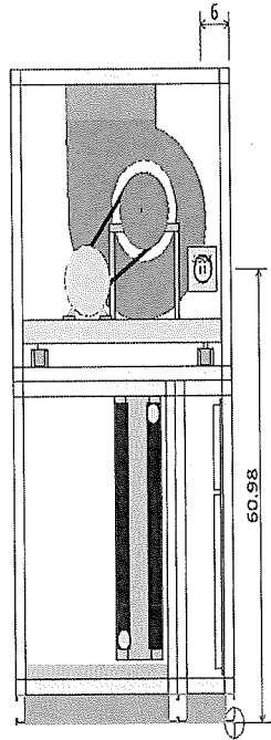
LEFT ELEVATION VIEW
