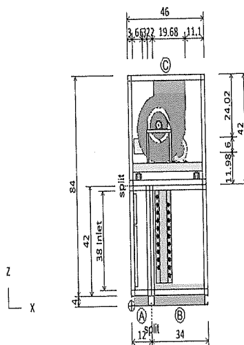
ELEVATION VIEW
