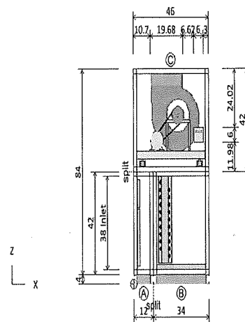
ELEVATION VIEW
