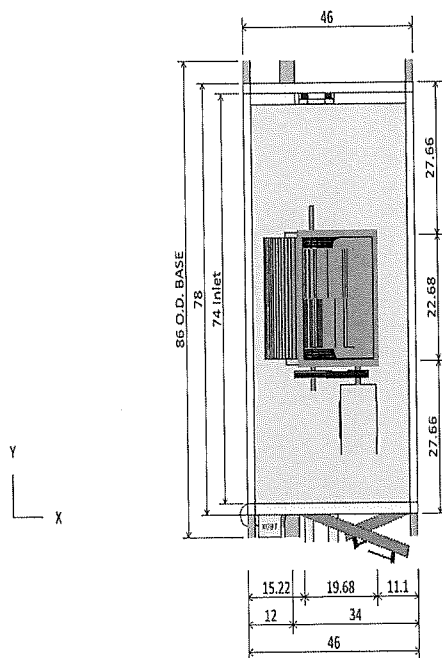
PLAN VIEW
