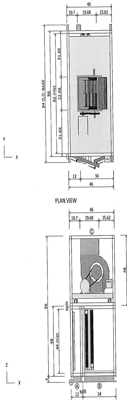
ELEVATION VIEW
