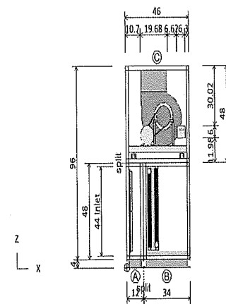
ELEVATION VIEW
