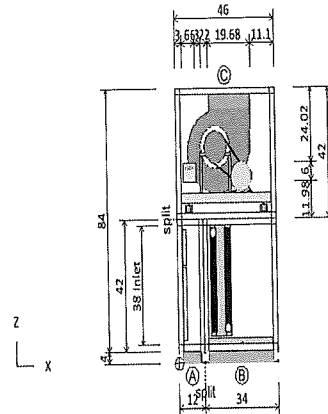
ELEVATION VIEW
